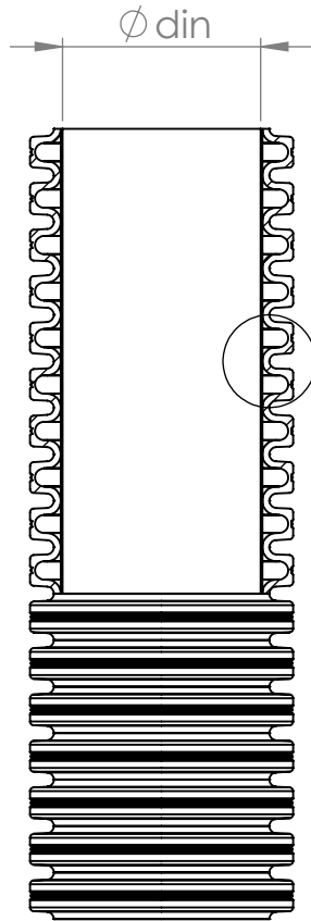
SECTION F-F
